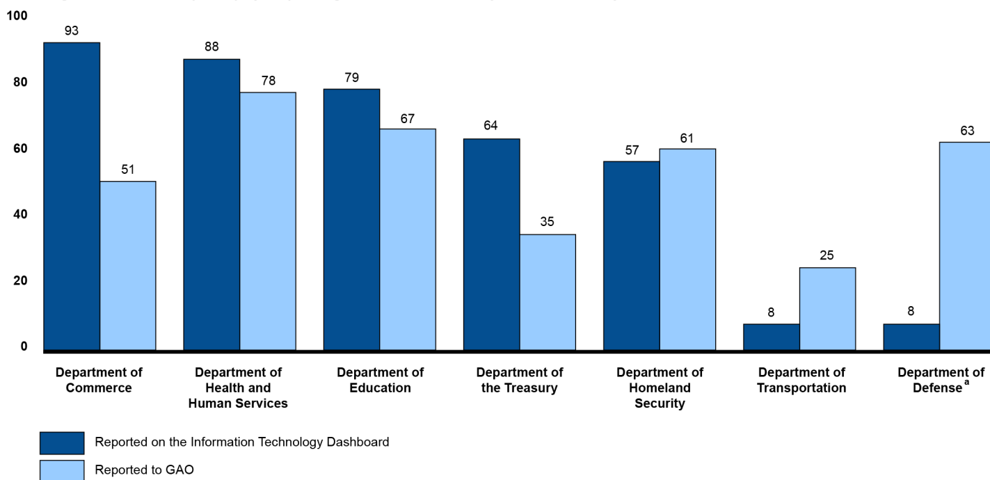
Figure 4: Comparison of Software Development Projects' Percentage of Planned Delivery Every 6 Months Reported on Information Technology (IT) Dashboard and to GAO for Fiscal Year 2016
